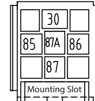
Relay Pin Locations As Viewed From The Wire Side of the Socket
