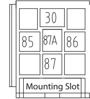
Relay Pin Locations As Viewed From The Wire Side of the Socket
